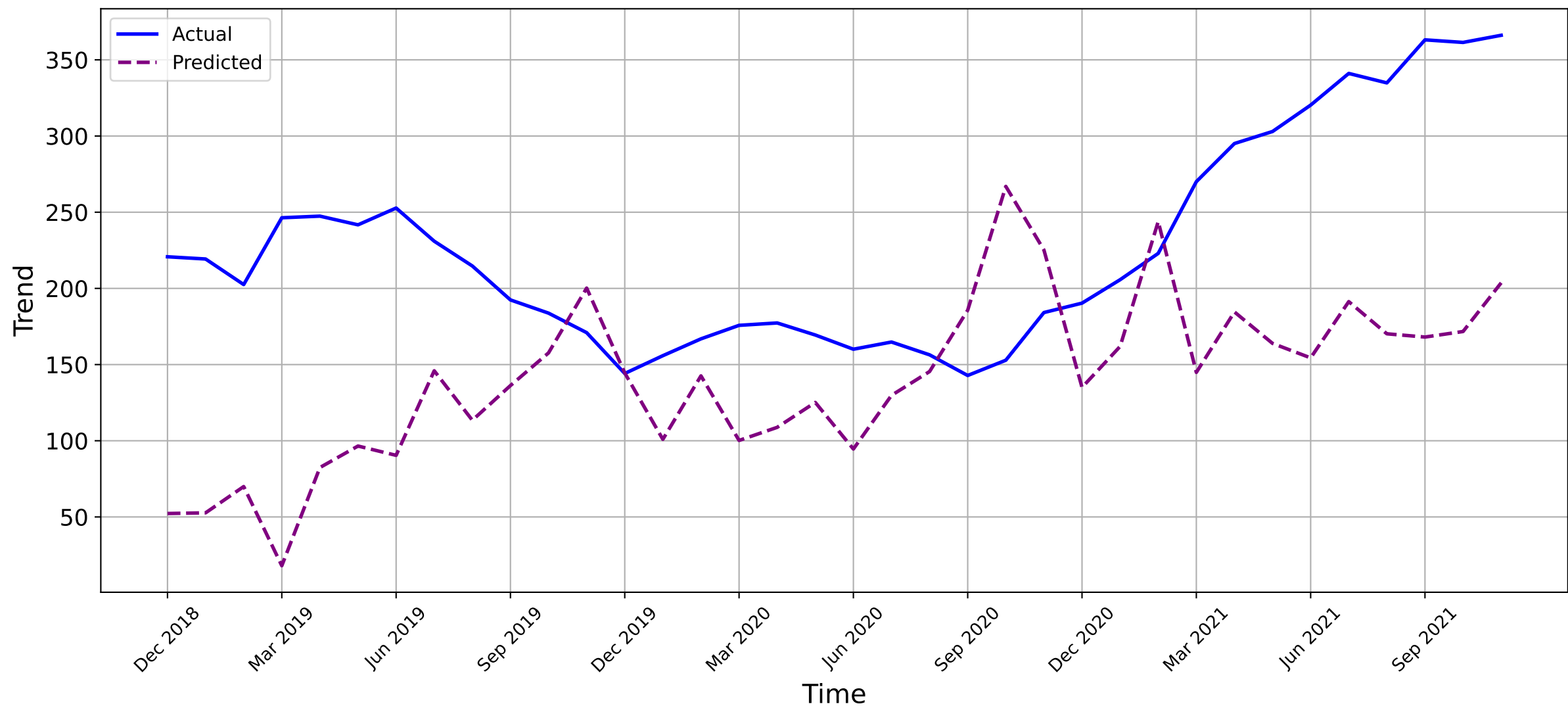
Vulnerability-ALL - Validation
